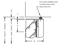
658. STANDARD HEAD DETAIL
