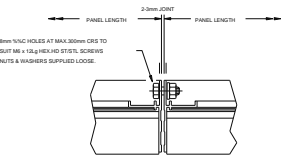
653. HORIZONTAL JOINT DETAIL
