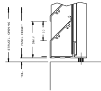
659. VARI-BLADE CILL DETAIL
