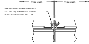
653. HORIZONTAL JOINT DETAIL
