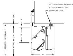
650. STANDARD HEAD DETAIL
