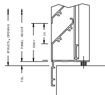
651. VARI-BLADE CILL DETAIL
